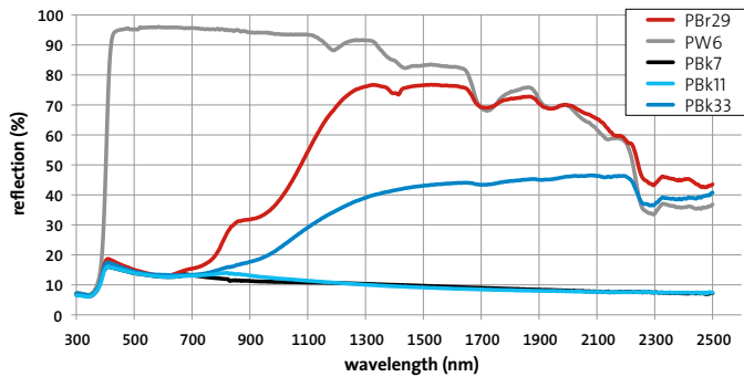
Figure 2: Reflection curves of different pigments
